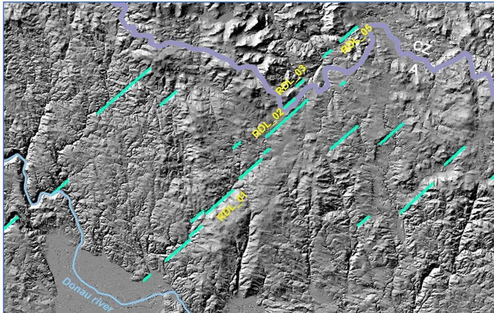
Fig. 1: Topo-lineaments related to the Rodl fault zone.
