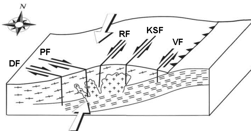
Fig. 2: Initial shear zone activity in the Danube (DF), Pfahl (PF), Rodl (RF), Karlstift (KSF) and Vitis (VF) Shear Zones. Arrows indicate major compression directions. Adopted from BRANDMAYR ET AL. (1997).
